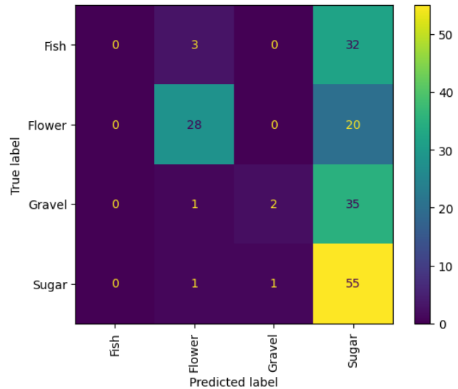
Testing dataset
