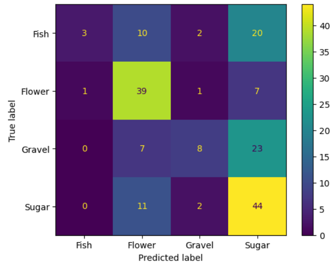
Testing dataset
