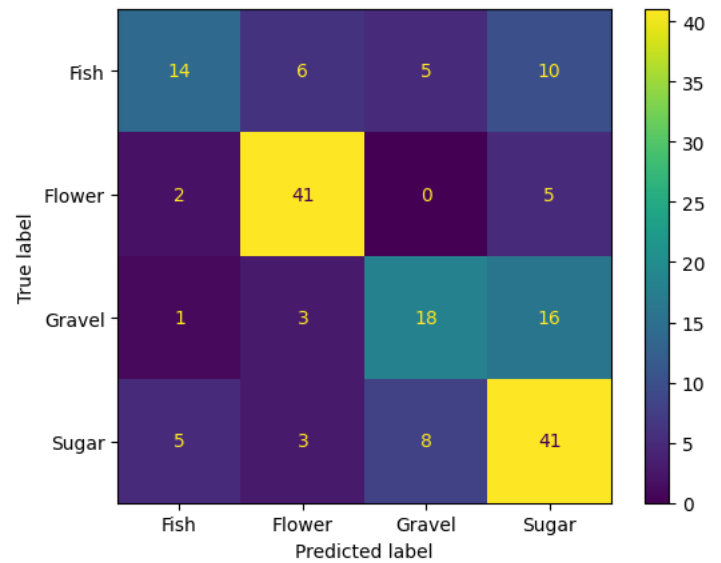
Testing dataset
